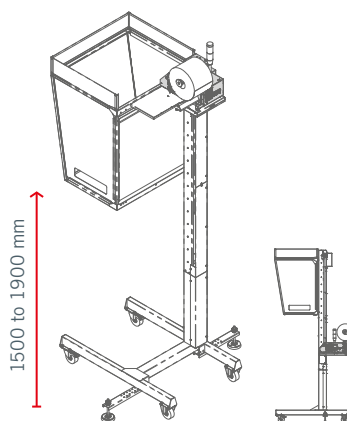
Electric overhead dispensing system code 50.2118
