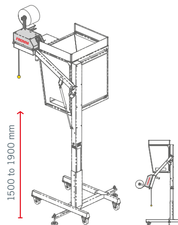
Manual overhead dispensing system code 50.2117
