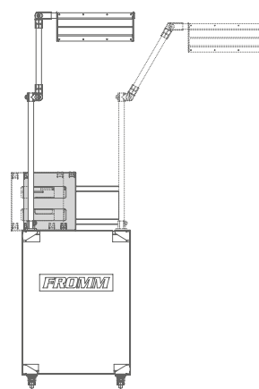
Compact mobile bin with articulated arm and pad holder code 50.2119
